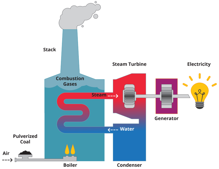
Figure 2. Figure Steam Turbine (coal)
